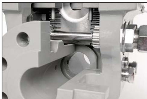
With orifice plate out of flow line
