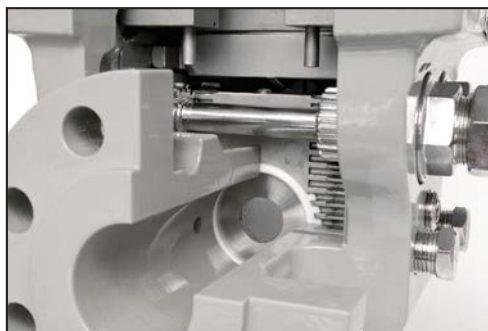
With orifice plate in flow line
